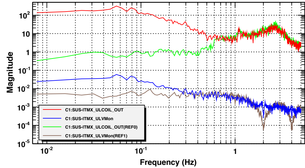
Power spectrum
