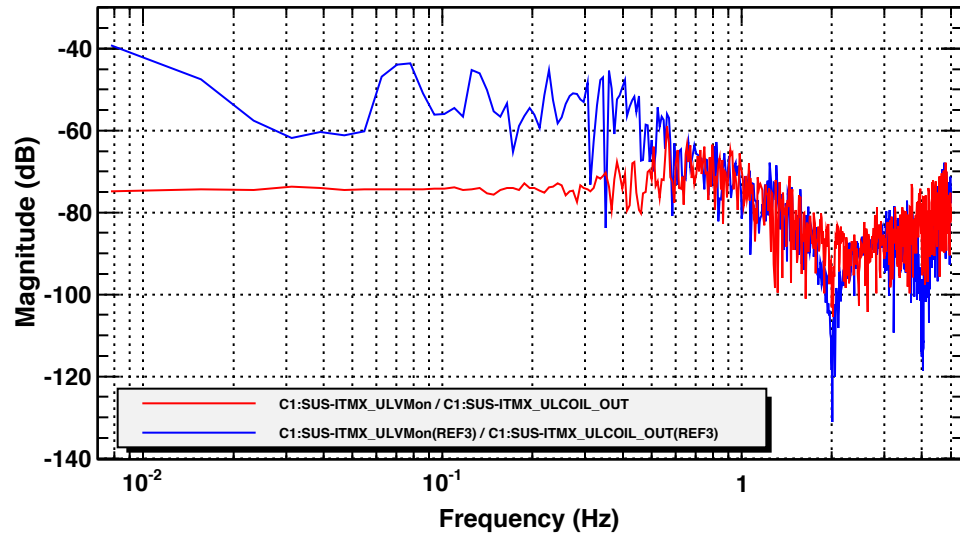
Transfer function
