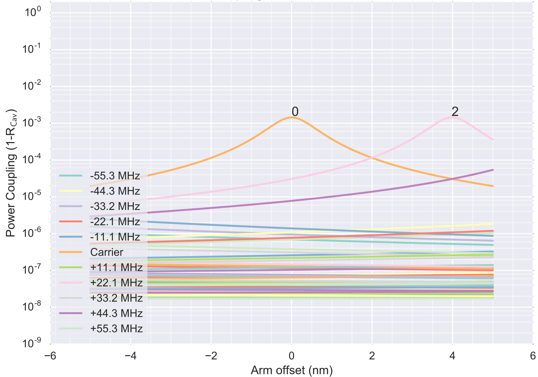
Power Coupling of HOMs into 40m X Arm
