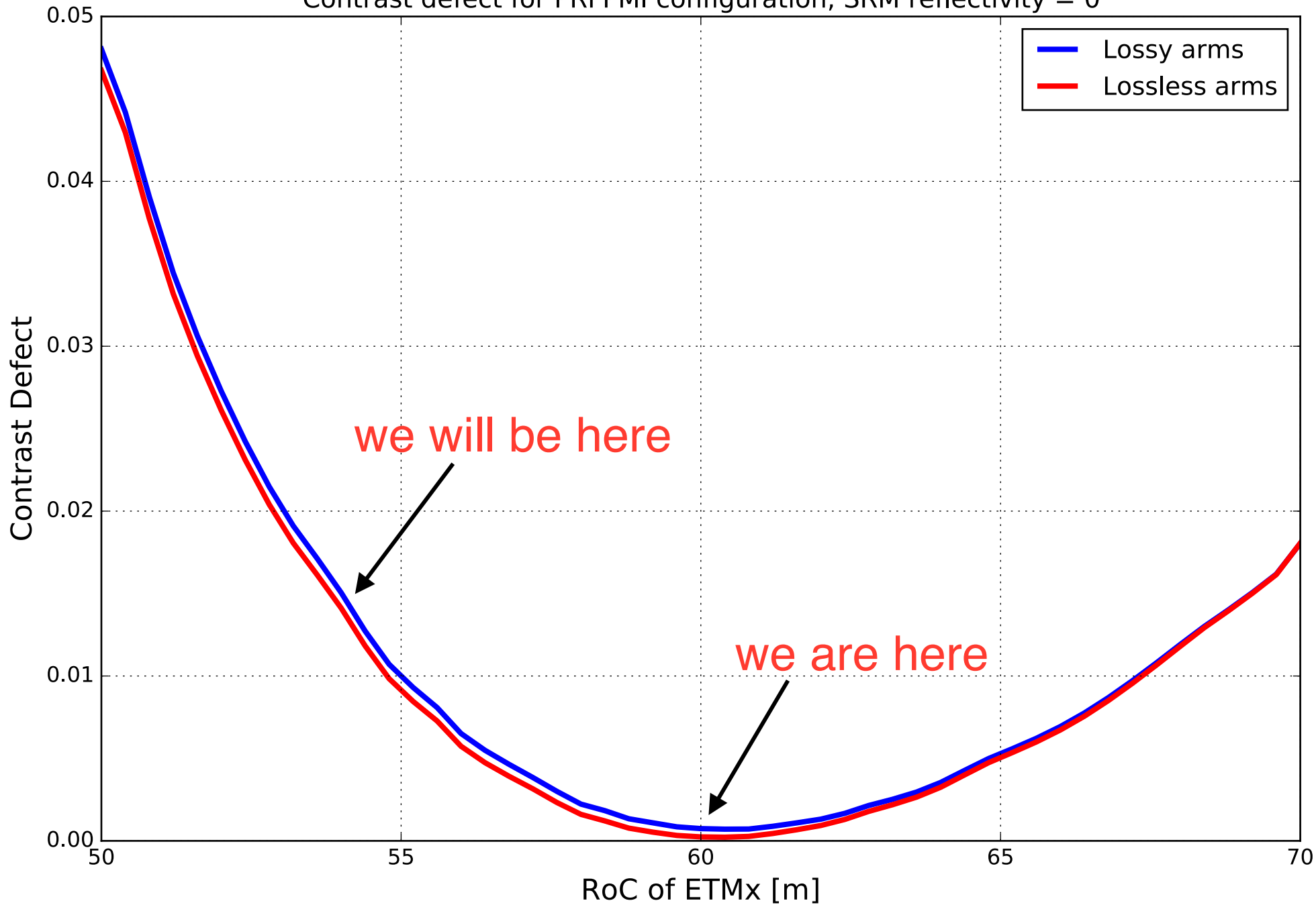
Contrast defect for PRFPMI configuration, SRM reflectivity = 0
