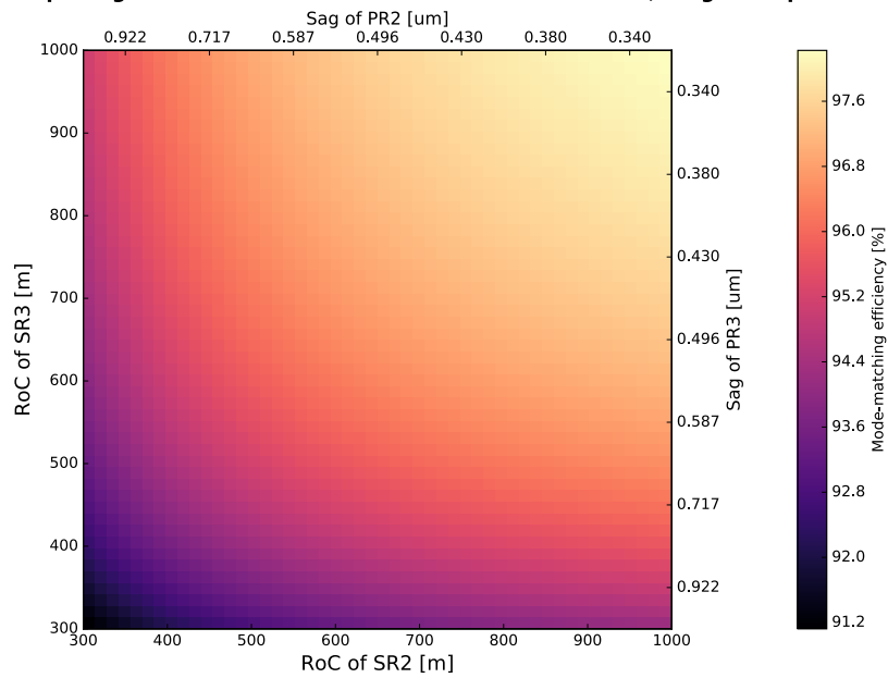
le-overlap integral evaluated between SRY and YARM cavities, tangential plane
