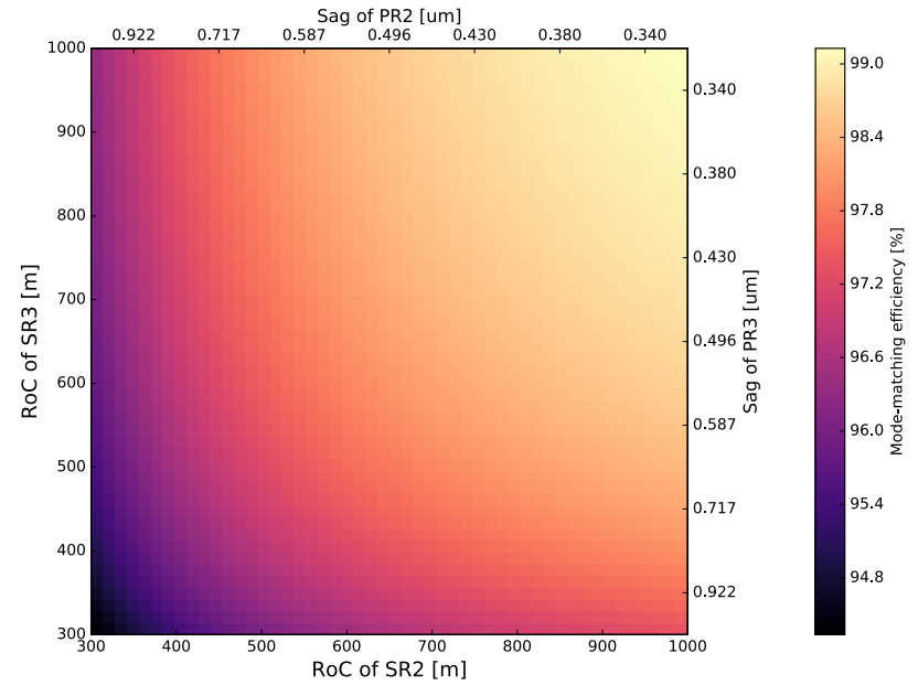
ode-overlap integral evaluated between SRX and XARM cavities, sagittal plane
