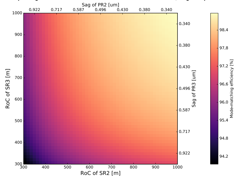
ode-overlap integral evaluated between SRY and YARM cavities, sagittal plane
