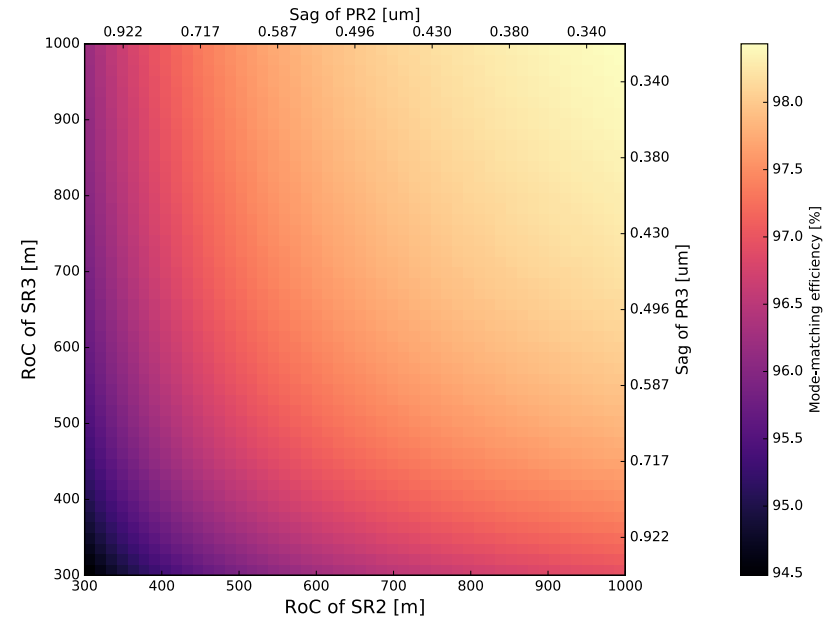
ode-overlap integral evaluated between PRX and XARM cavities, sagittal plane
