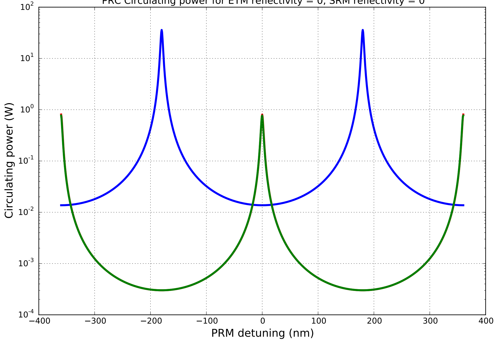
PRC Circulating power for ETM reflectivity = 0, SRM reflectivity = 0
