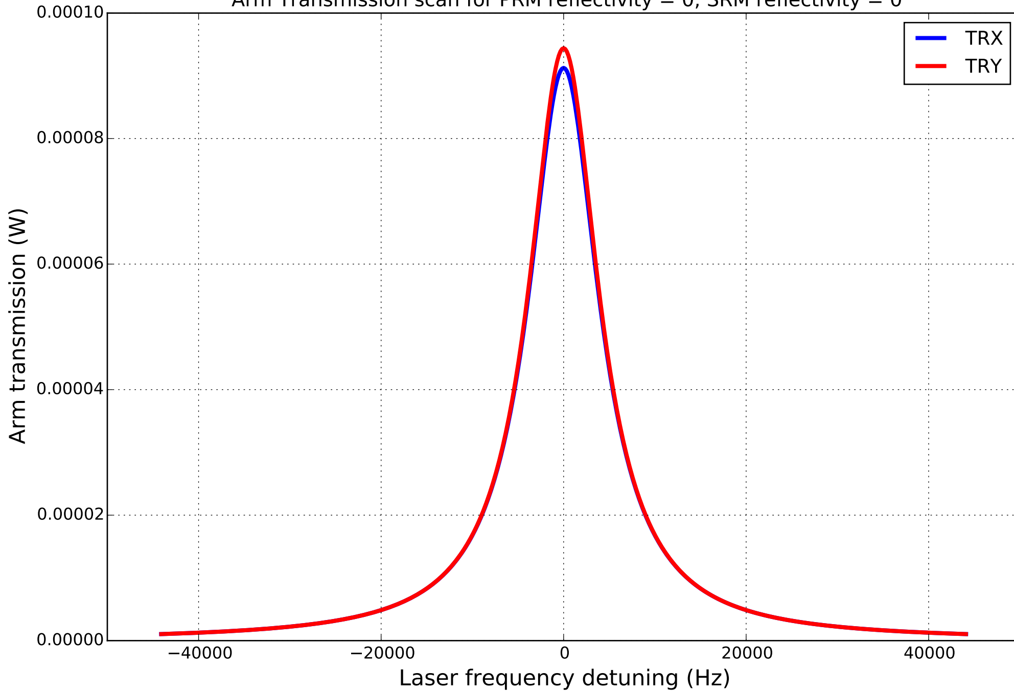
Arm Transmission scan for PRM reflectivity = 0, SRM reflectivity = 0
