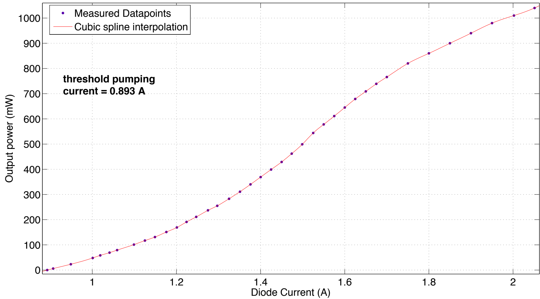
Output power vs diode pumping current for 40m 1W Innolight NPRO (17 April 2016)
