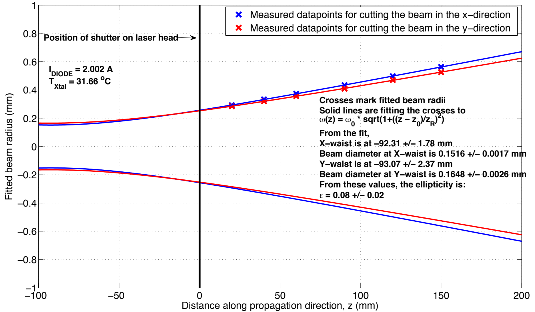
Beam profiling 40m 1W Innolight NPRO: z-scan results (17 April 2016)
