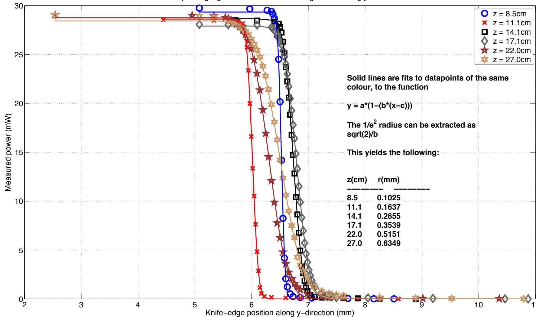
Beam profiling Lightwave NPRO – Knife-edge scans along y-direction
