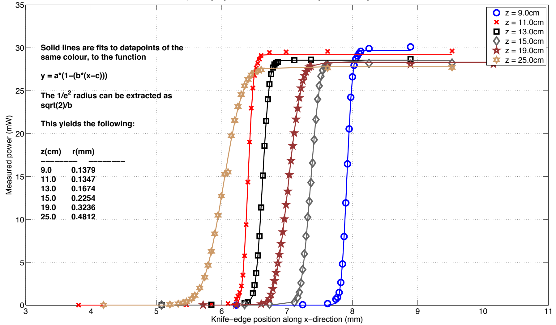
Beam profiling Lightwave NPRO – Knife-edge scans along x-direction
