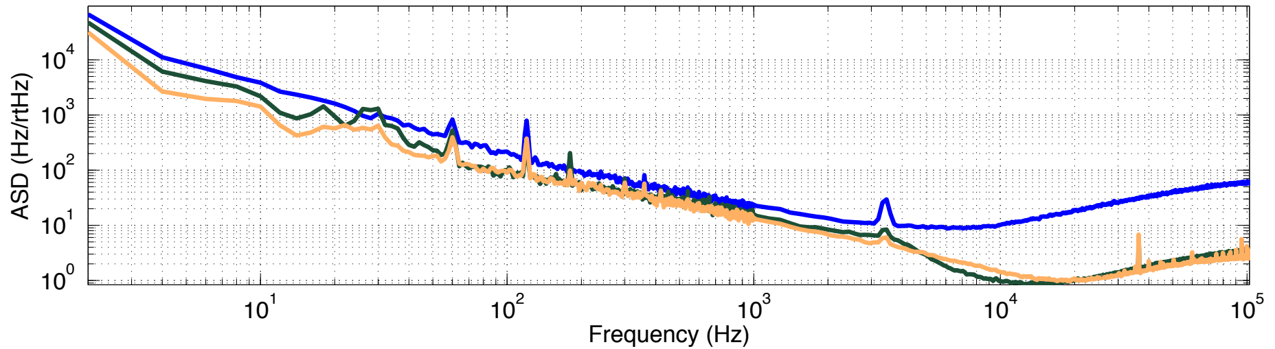
Comparison of frequency noise of Innolight, Lightwave and Spare Innolight – Calibrated
