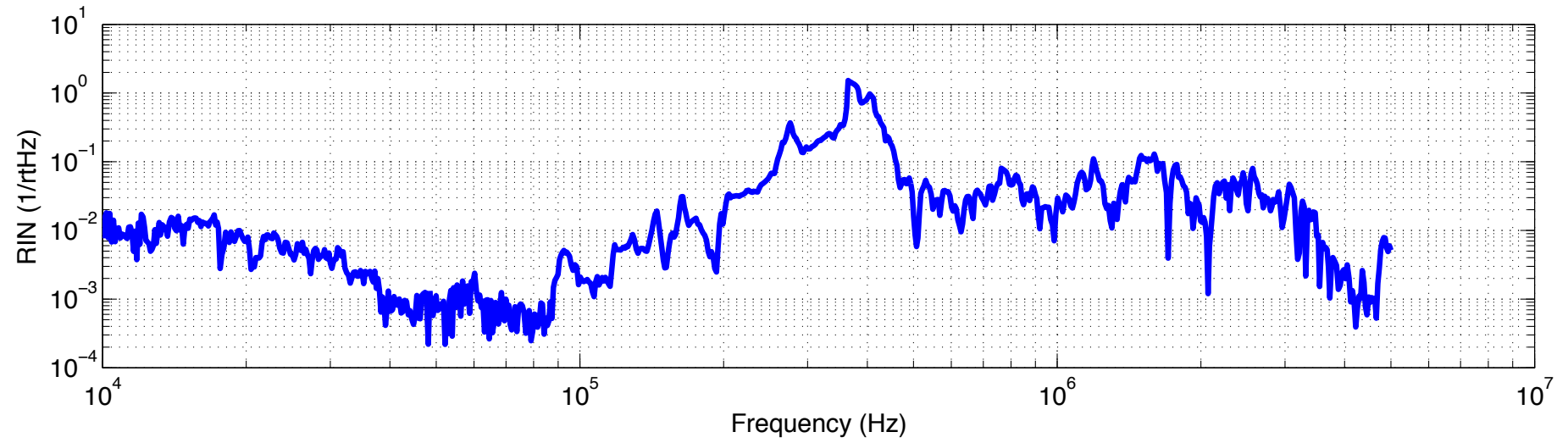
AM response of AUX X Laser (Innolight)
