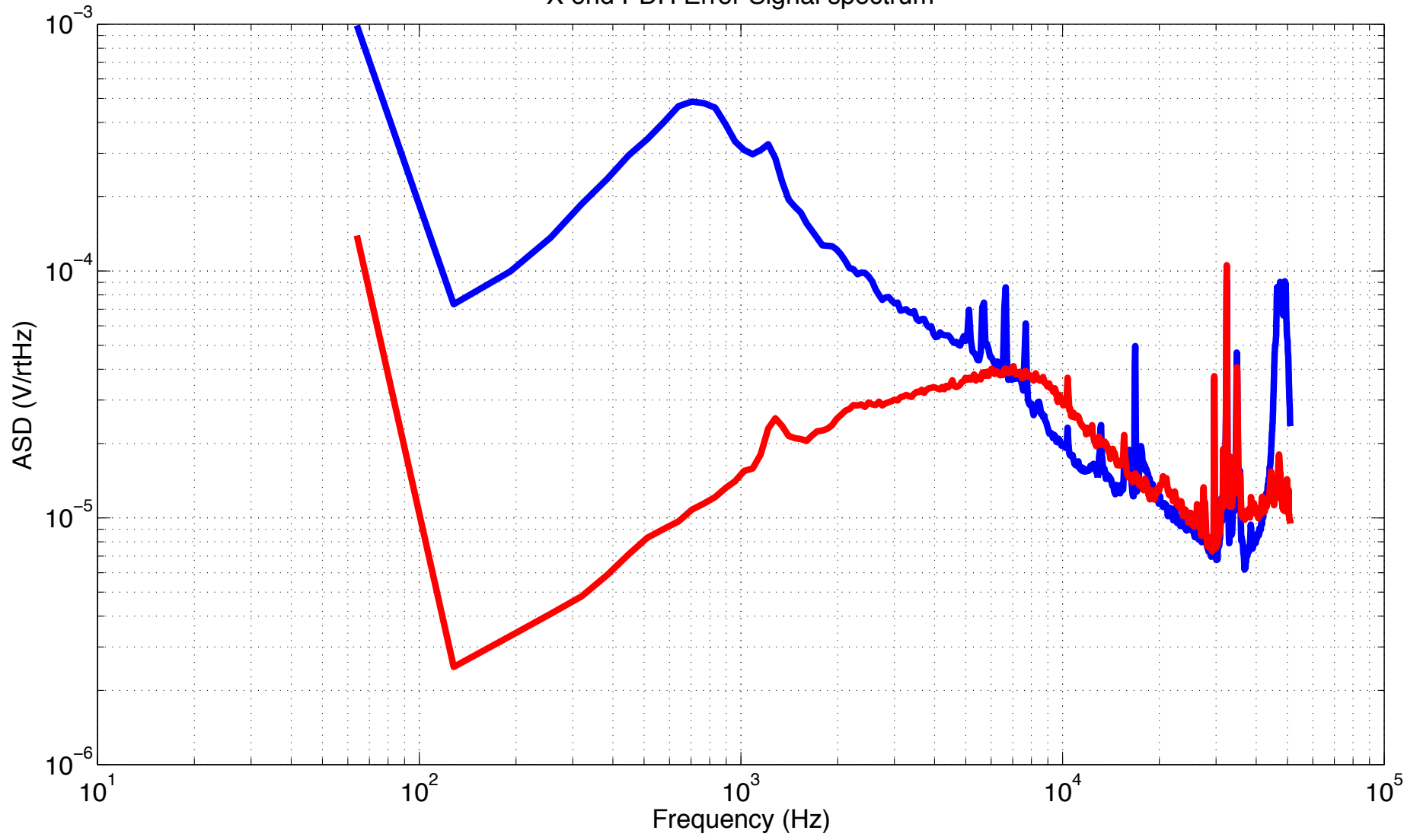
X end PDH Error Signal spectrum
