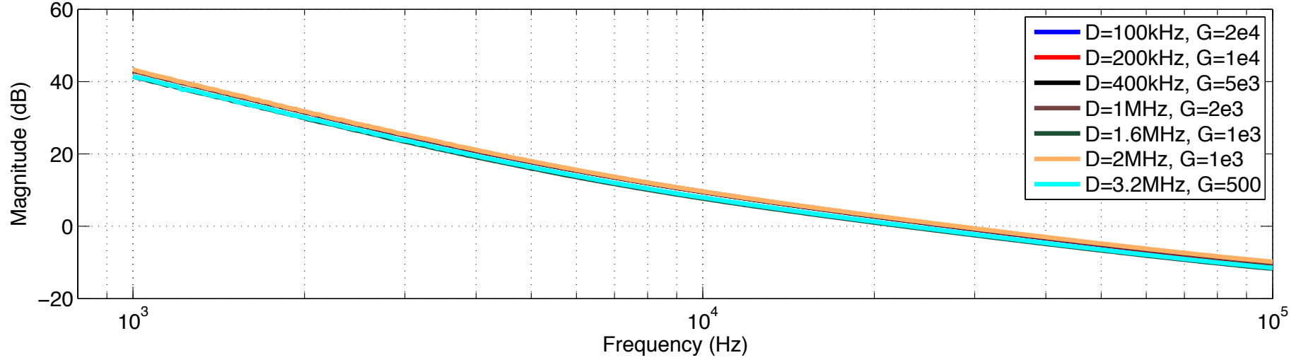
Measured PLL OLGs for Marconi 2023B (LO) locked to 2023A ("Beat" Source)
