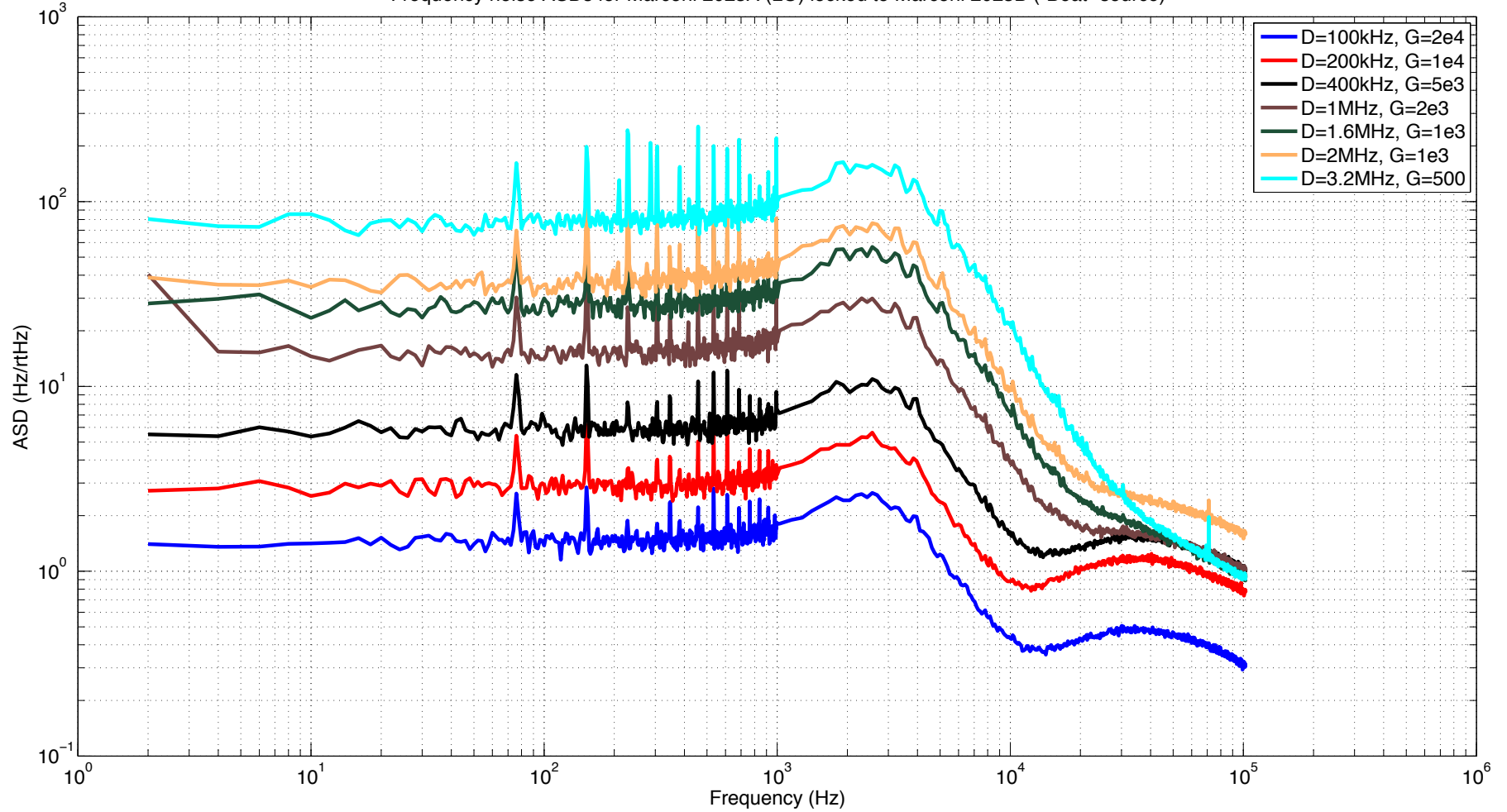
Frequency noise ASDs for Marconi 2023A (LO) locked to Marconi 2023B ("Beat" source)
