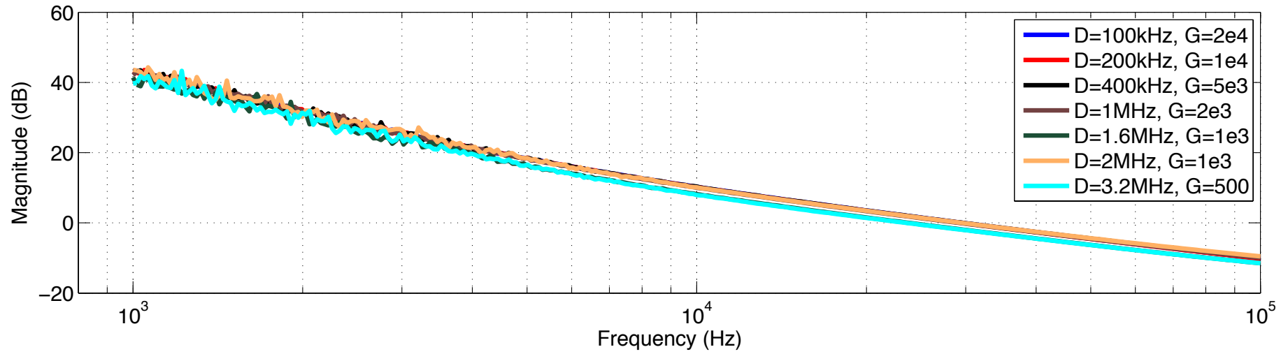
Measured PLL OLGs for Marconi 2023A (LO) locked to Marconi 2023B ("Beat" Source)
