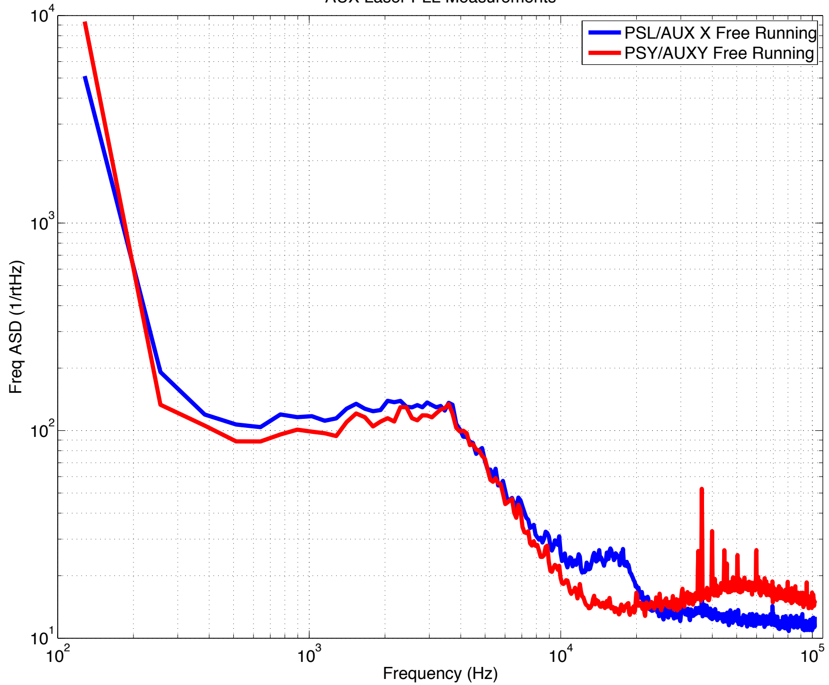
AUX Laser PLL Measurements
