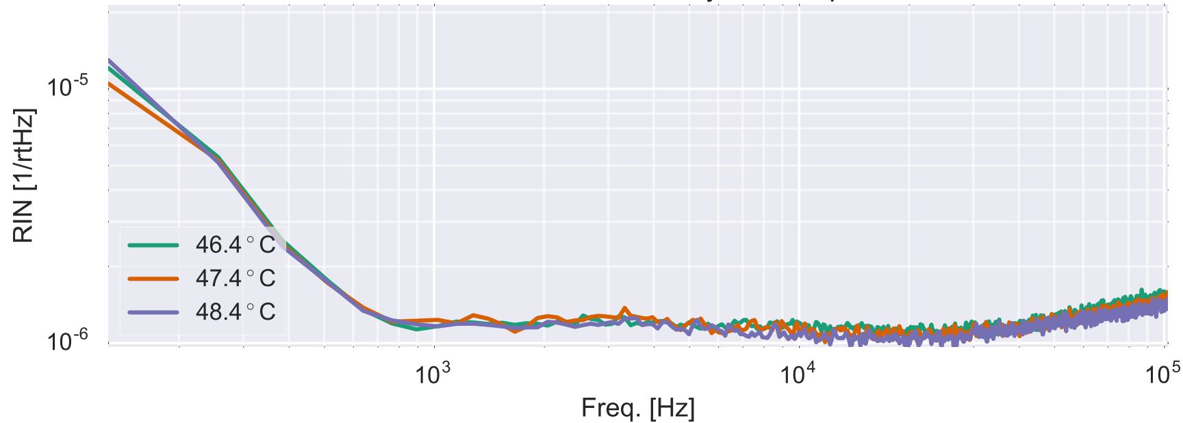
AUX X IR RIN with Crystal Temp
