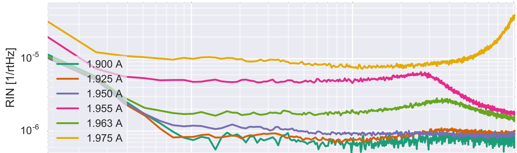
AUX X IR RIN with Diode Current
