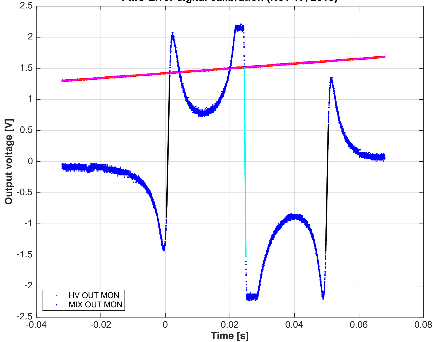
PMC Error signal calibration (Nov 17, 2015)
