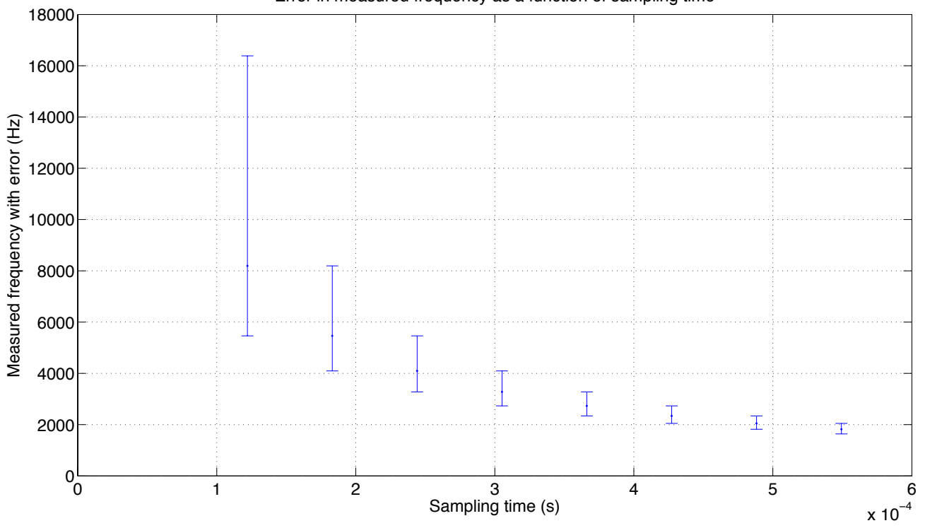
Error in measured frequency as a function of sampling time
