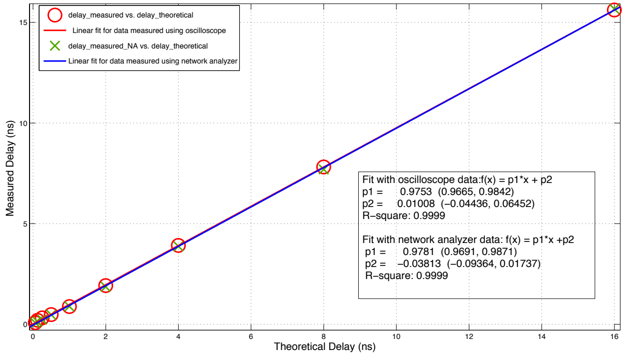
Checking Delay Line Phase Shifter (D050339)
