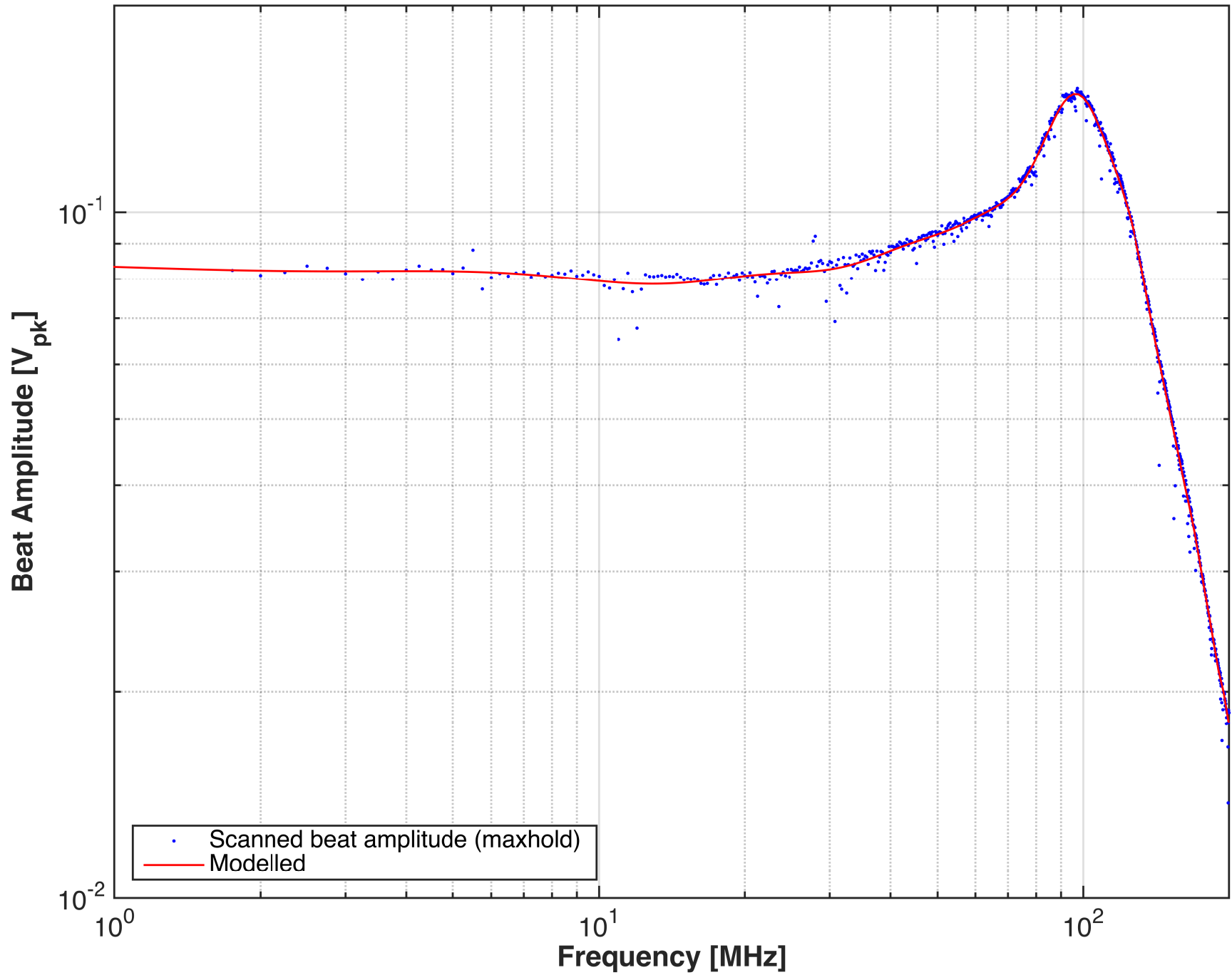
Photodetector response / PDA10CF
