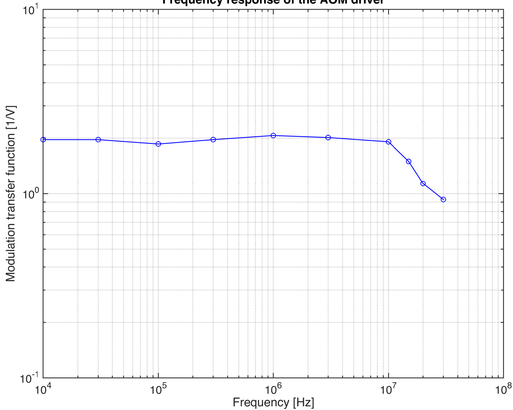
Frequency response of the AOM driver
