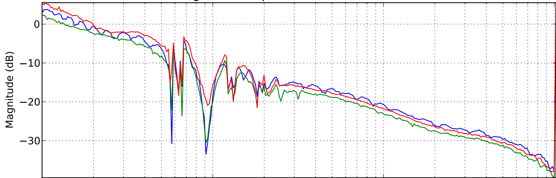
Analog CARM loop TF - Feb 03 2015 - 03:18:29
