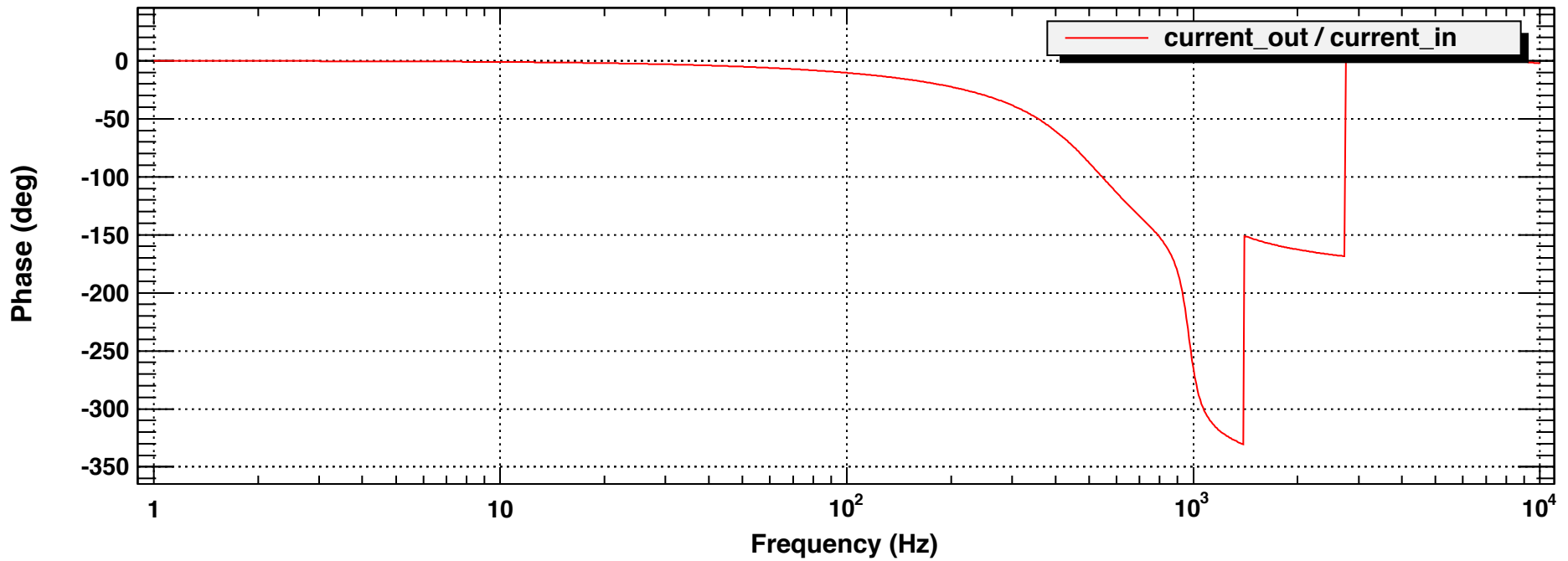
Transfer function
