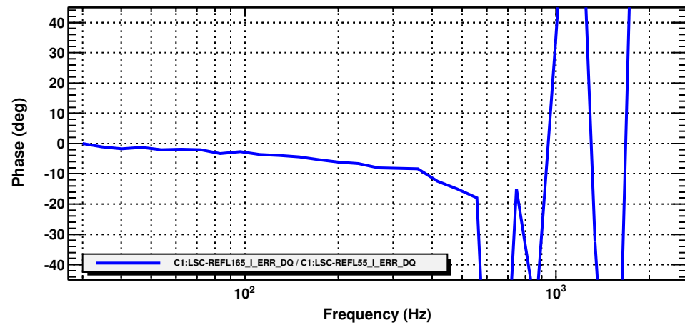
Transfer function
