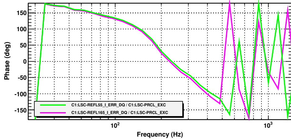
Transfer function
