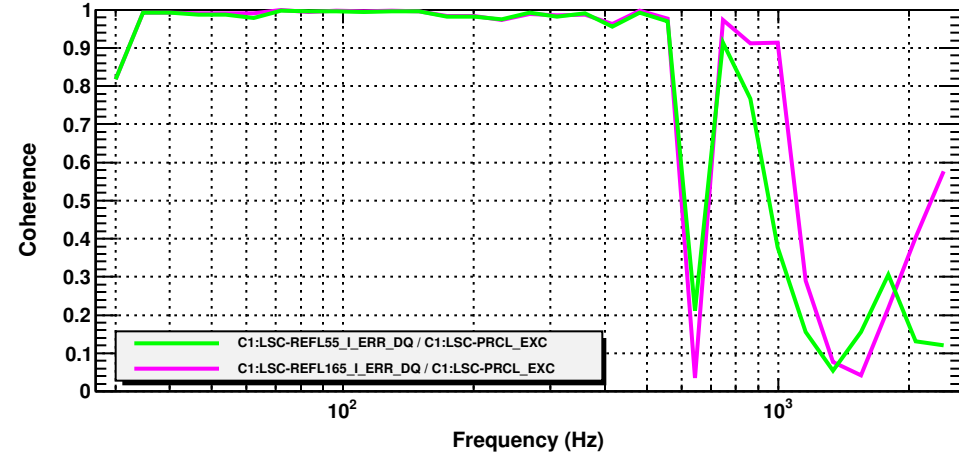
Coherence function
