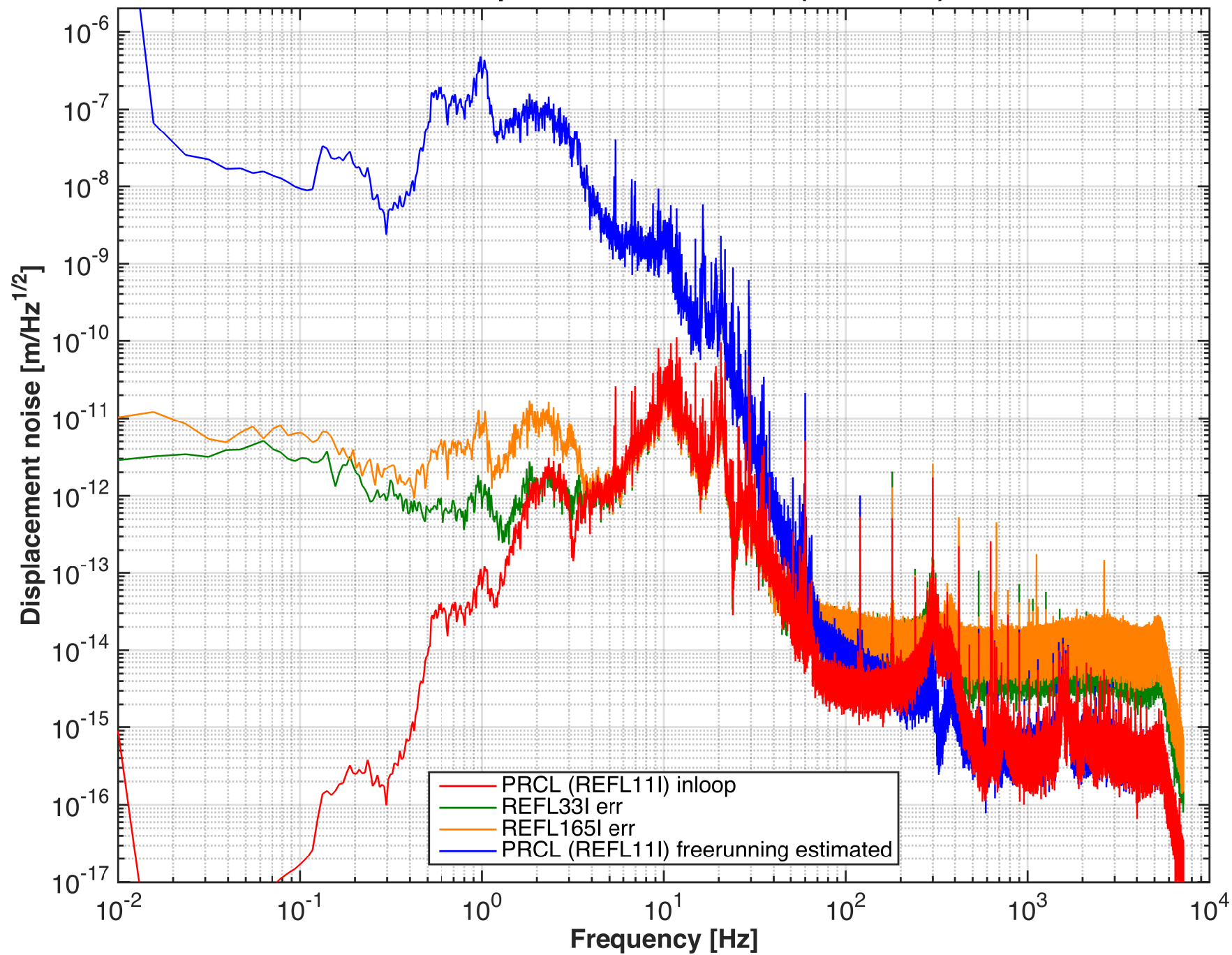
PRCL displacement noise / DRMI (2014/10/31)
