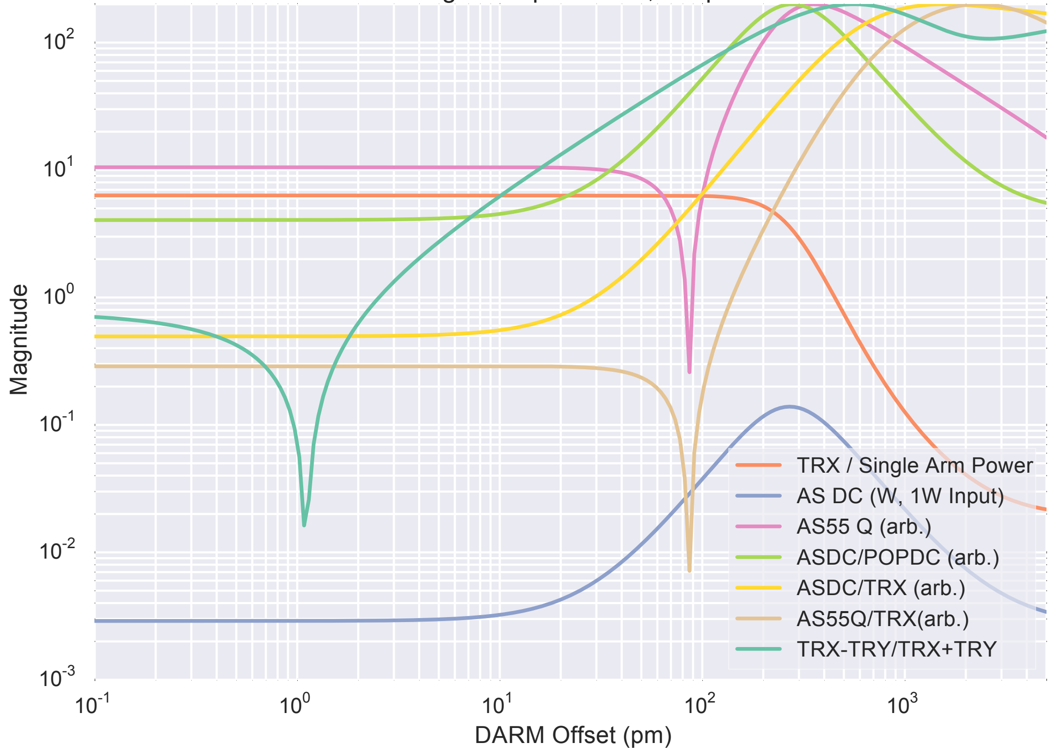
DARM Offset Signal Dependence, 120pm CARM offset
