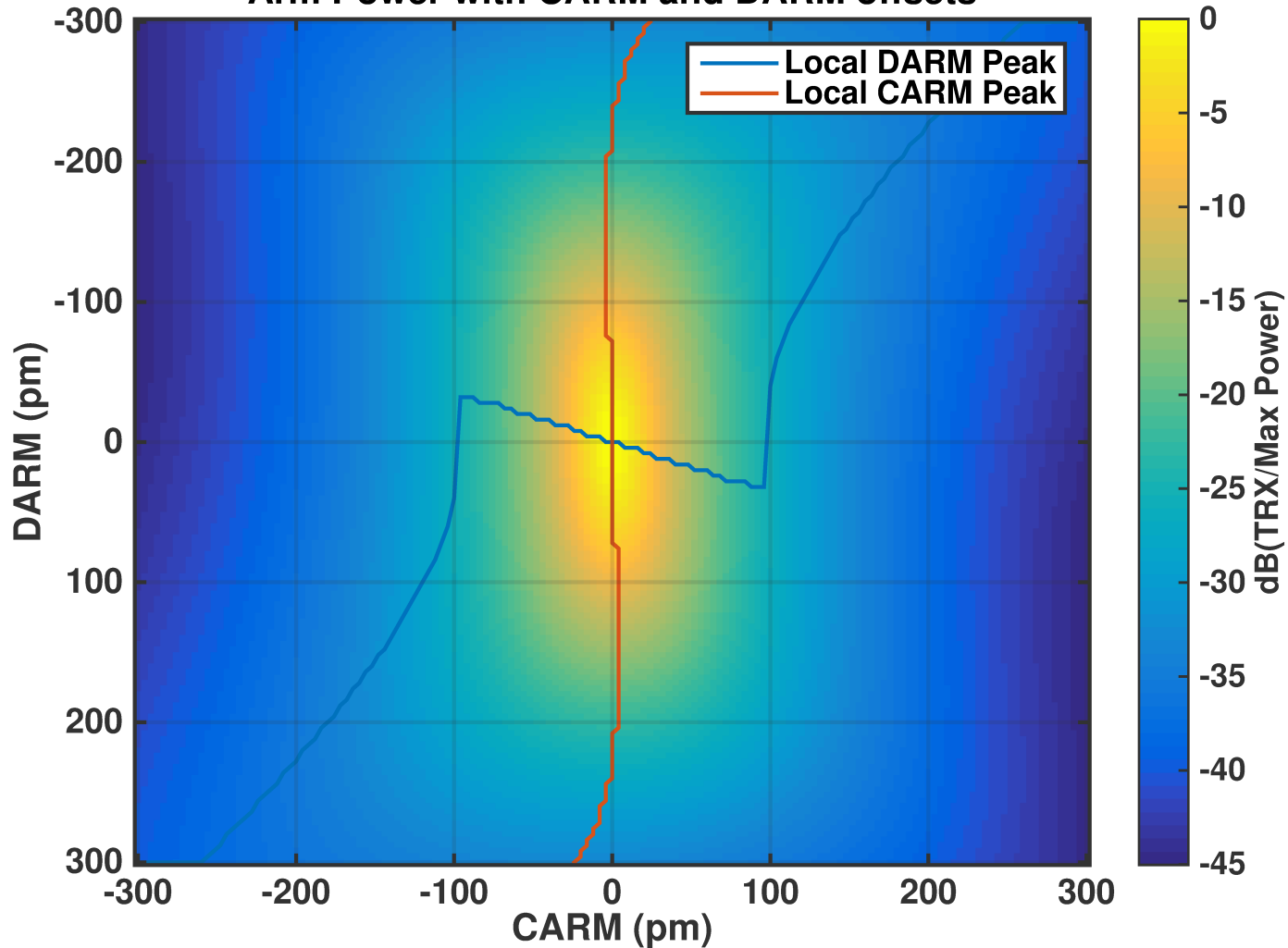
Arm Power with CARM and DARM offsets
