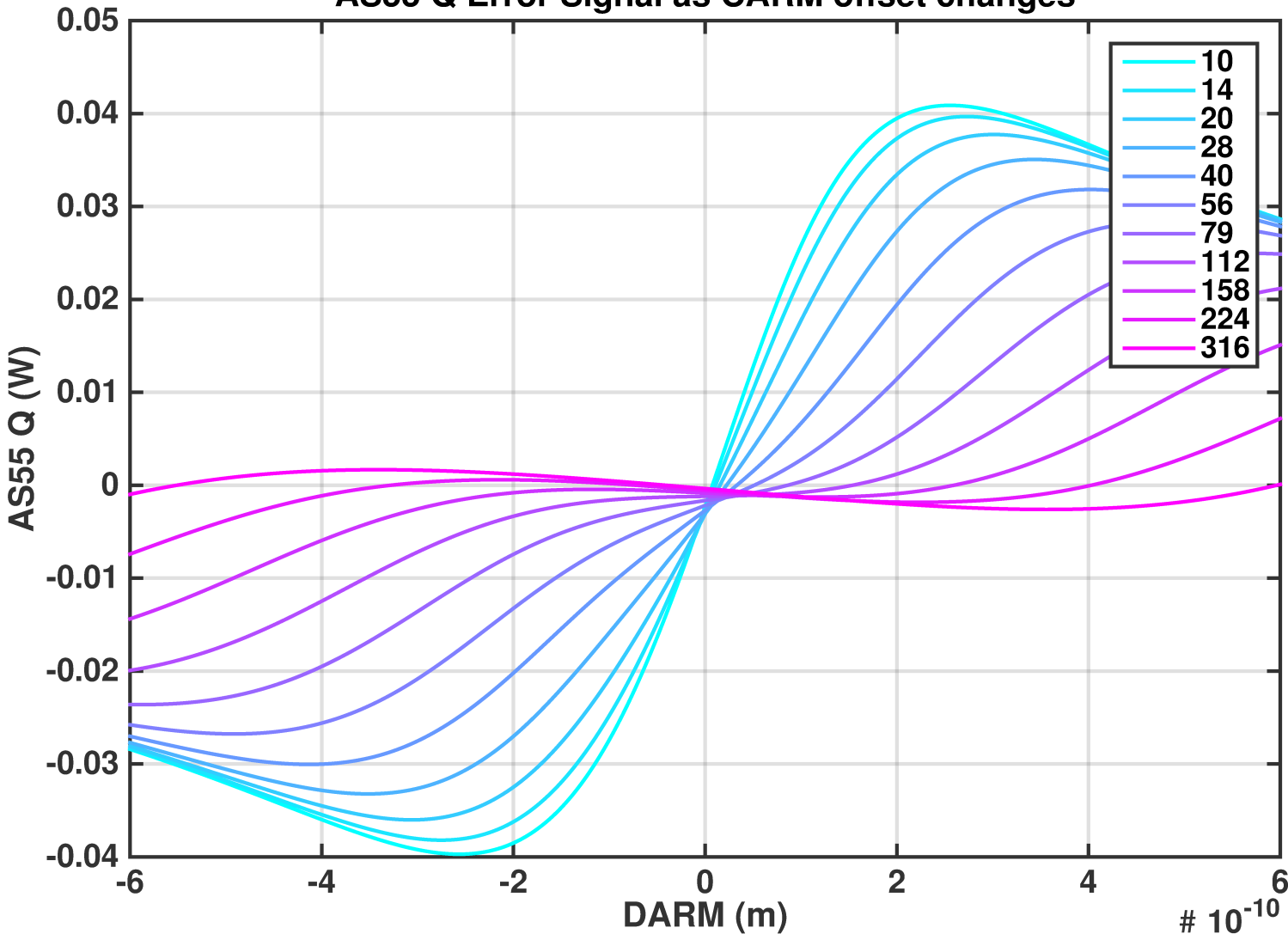
AS55 Q Error Signal as CARM offset changes
