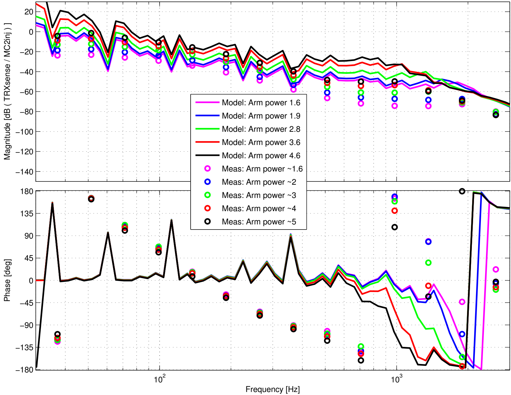
CARM Open Loop Gain, Model=spring, DigOffset=Neg
