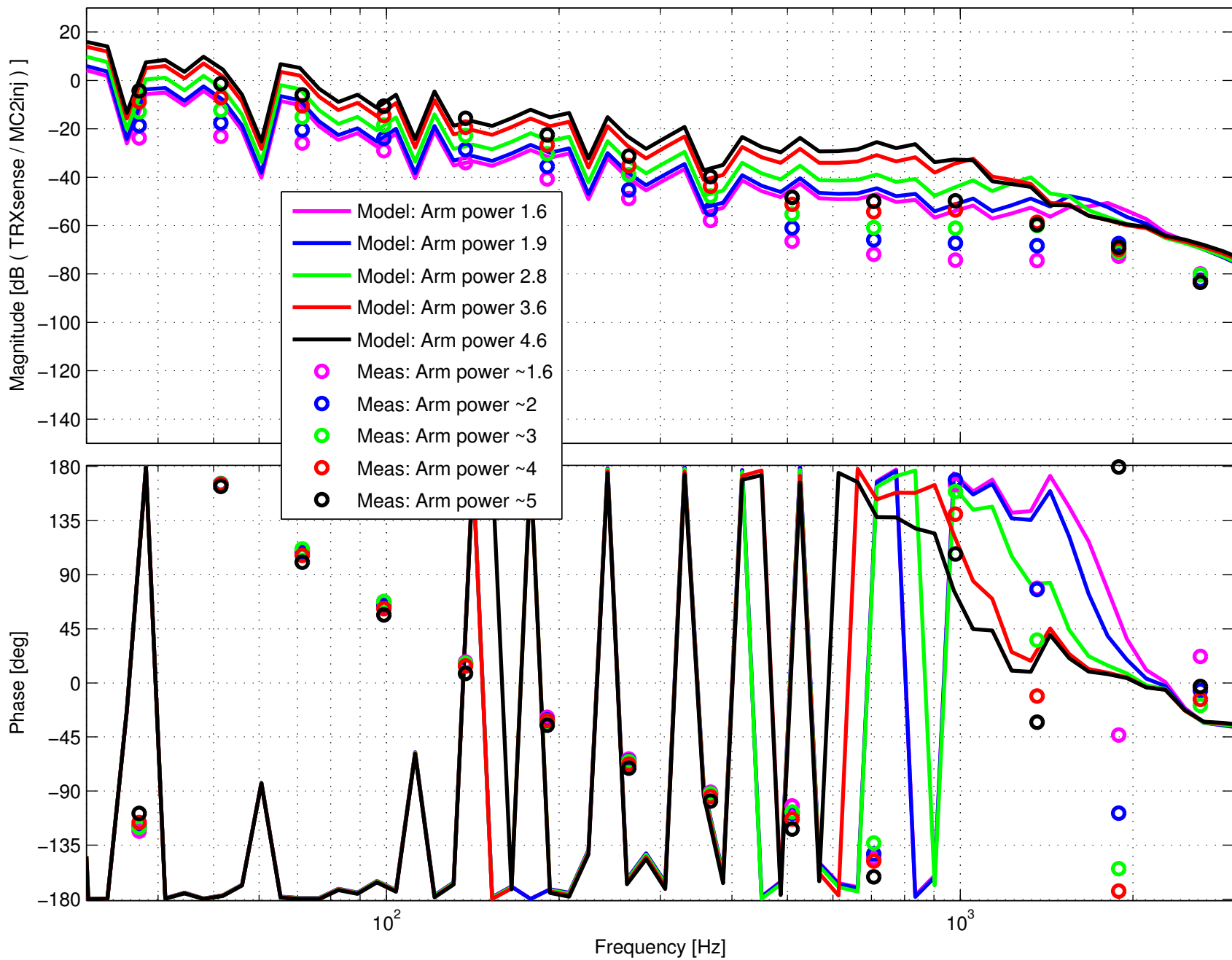
CARM Open Loop Gain, Model=antispring, DigOffset=Neg
