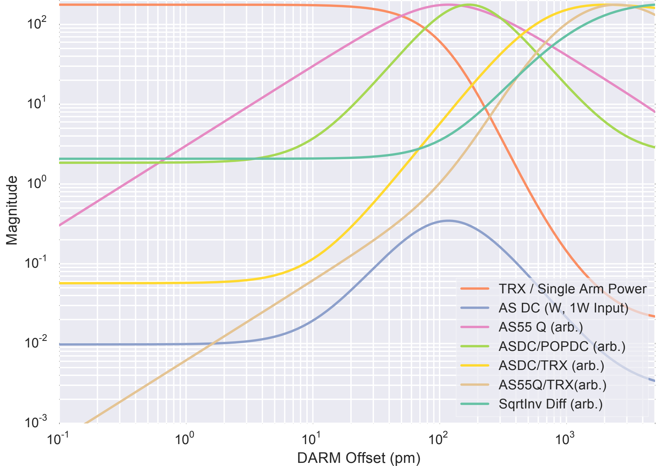
DARM Offset Signal Dependence, 0pm CARM offset
