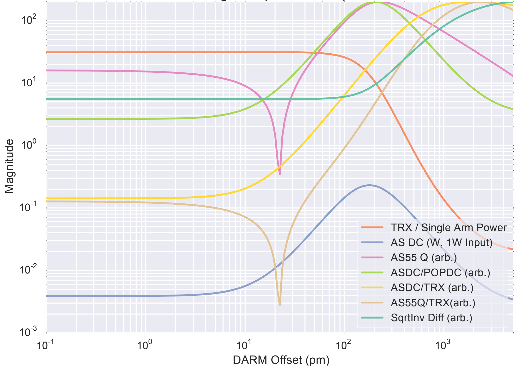
DARM Offset Signal Dependence, 50pm CARM offset
