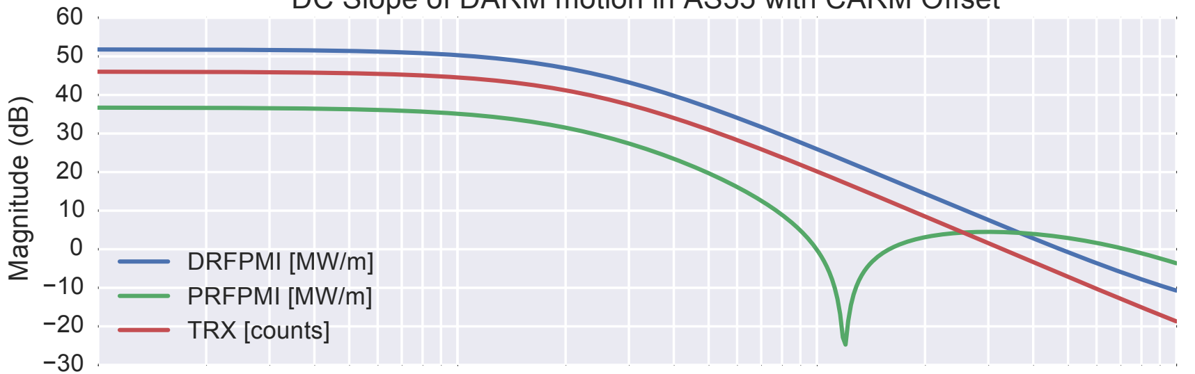
DC Slope of DARM motion in AS55 with CARM Offset
