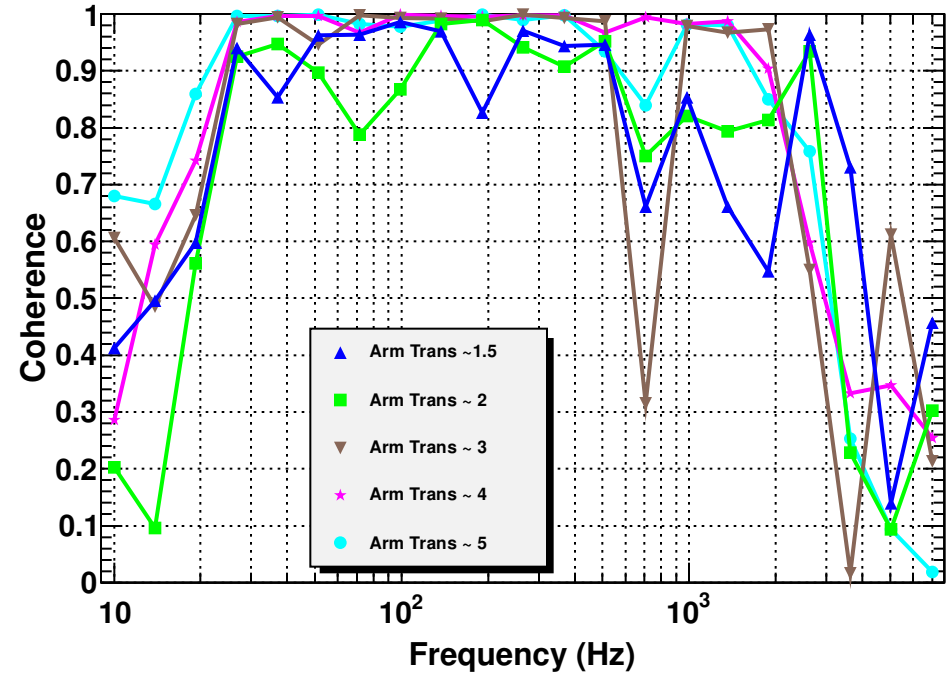
Coherence function
