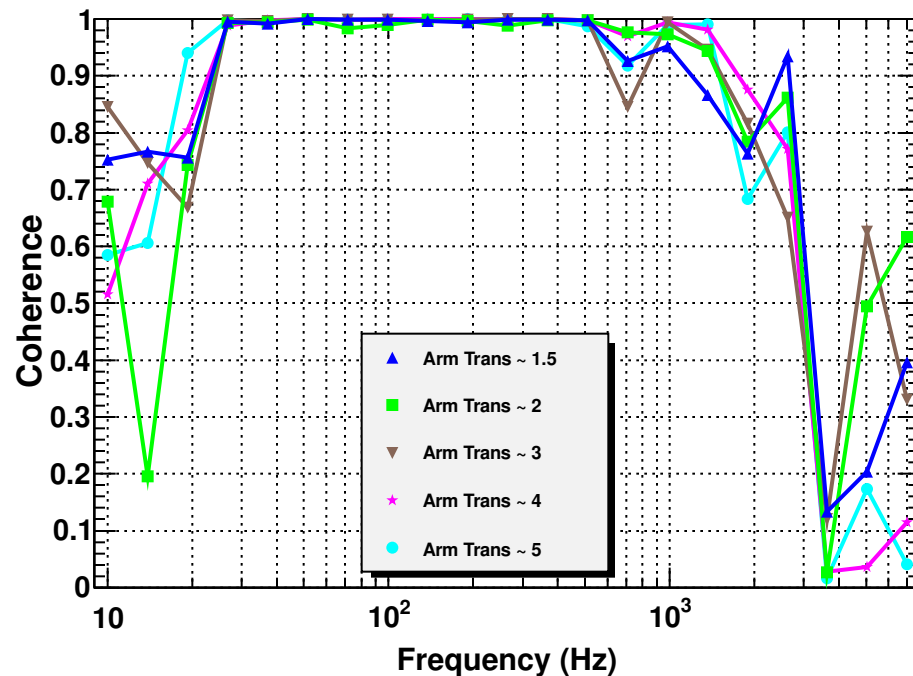
Coherence function
