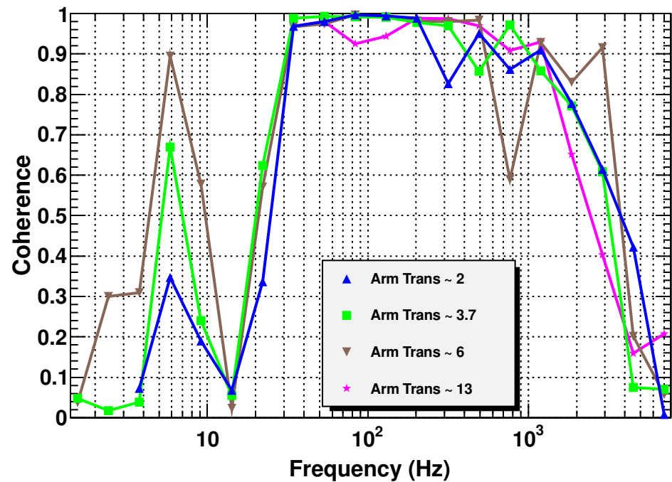
Coherence function
