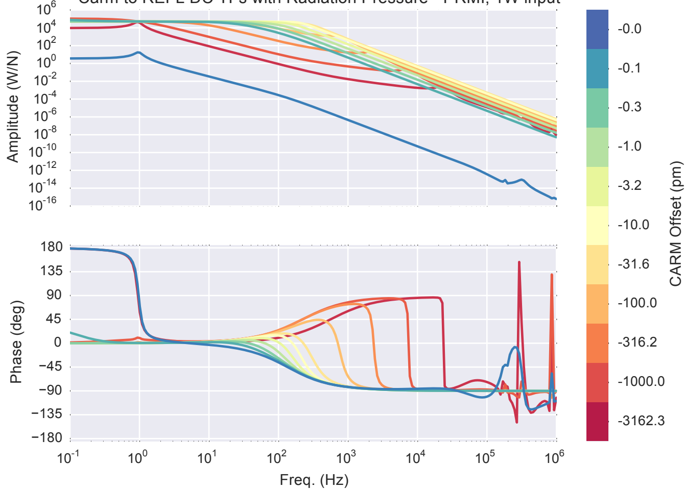
Carm to REFL DC TFs with Radiation Pressure - PRMI, 1W input
