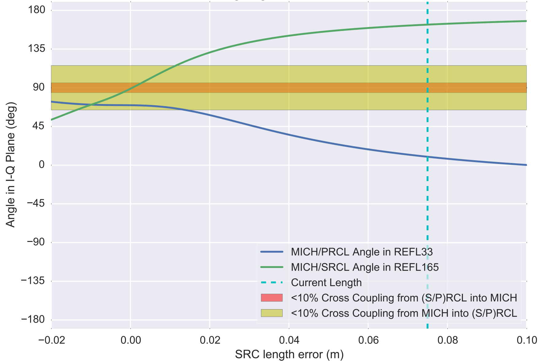
Relative MICH Sensing Angles in 3F RFPDs - Zero Carm Offset
