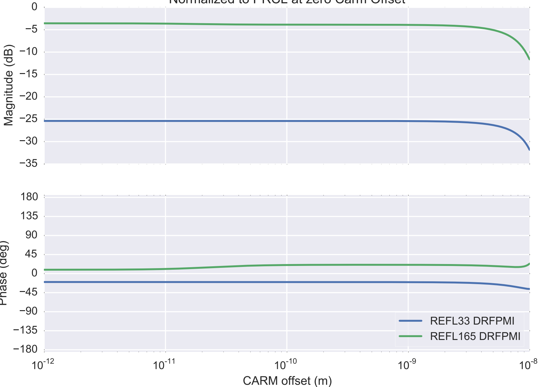
DC SRCL sensing in REFL 3F (Corrected SRC Length) Normalized to PRCL at zero CARM Offset
