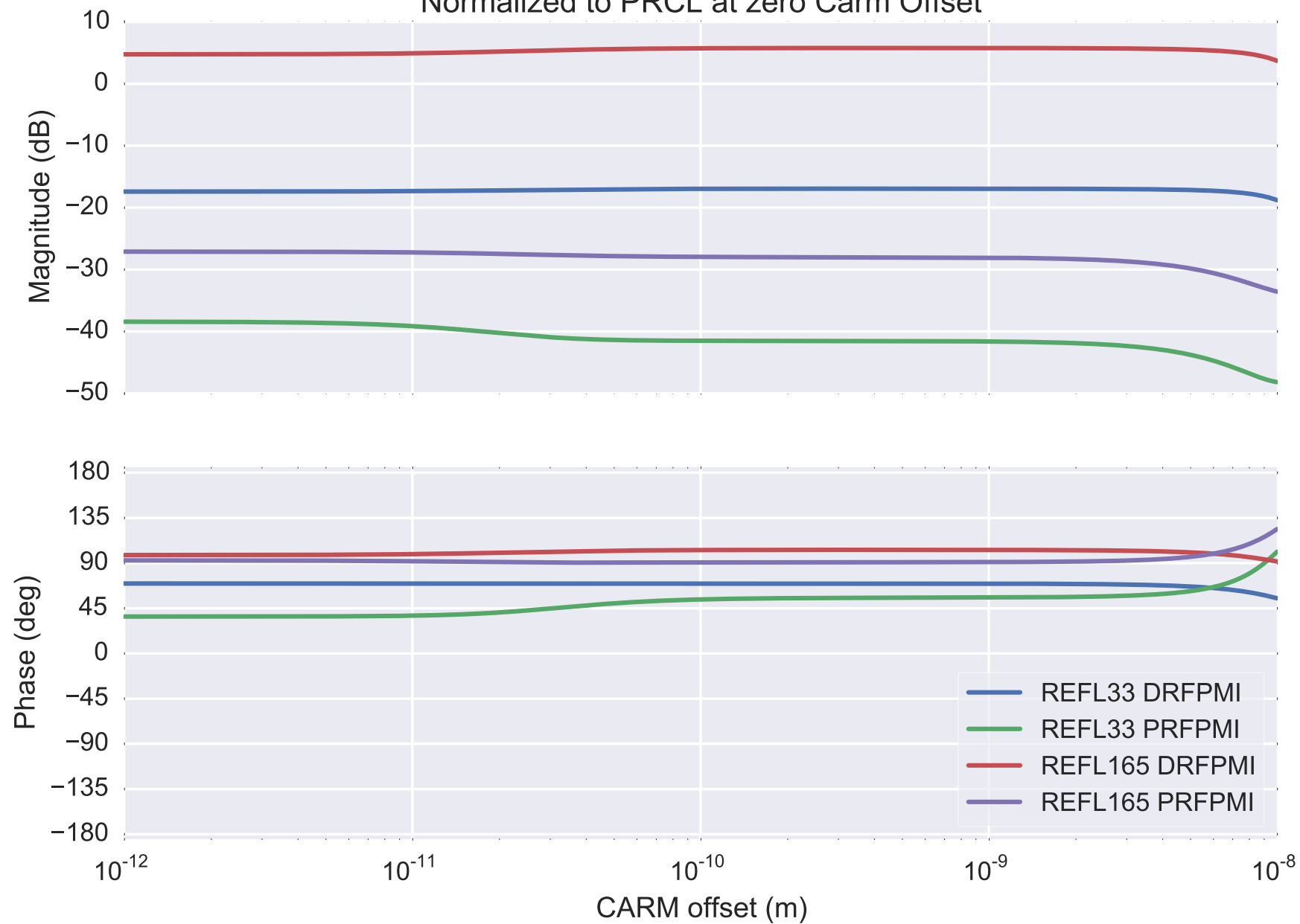
DC MICH sensing in REFL 3F (Corrected SRC Length) Normalized to PRCL at zero Carm Offset
