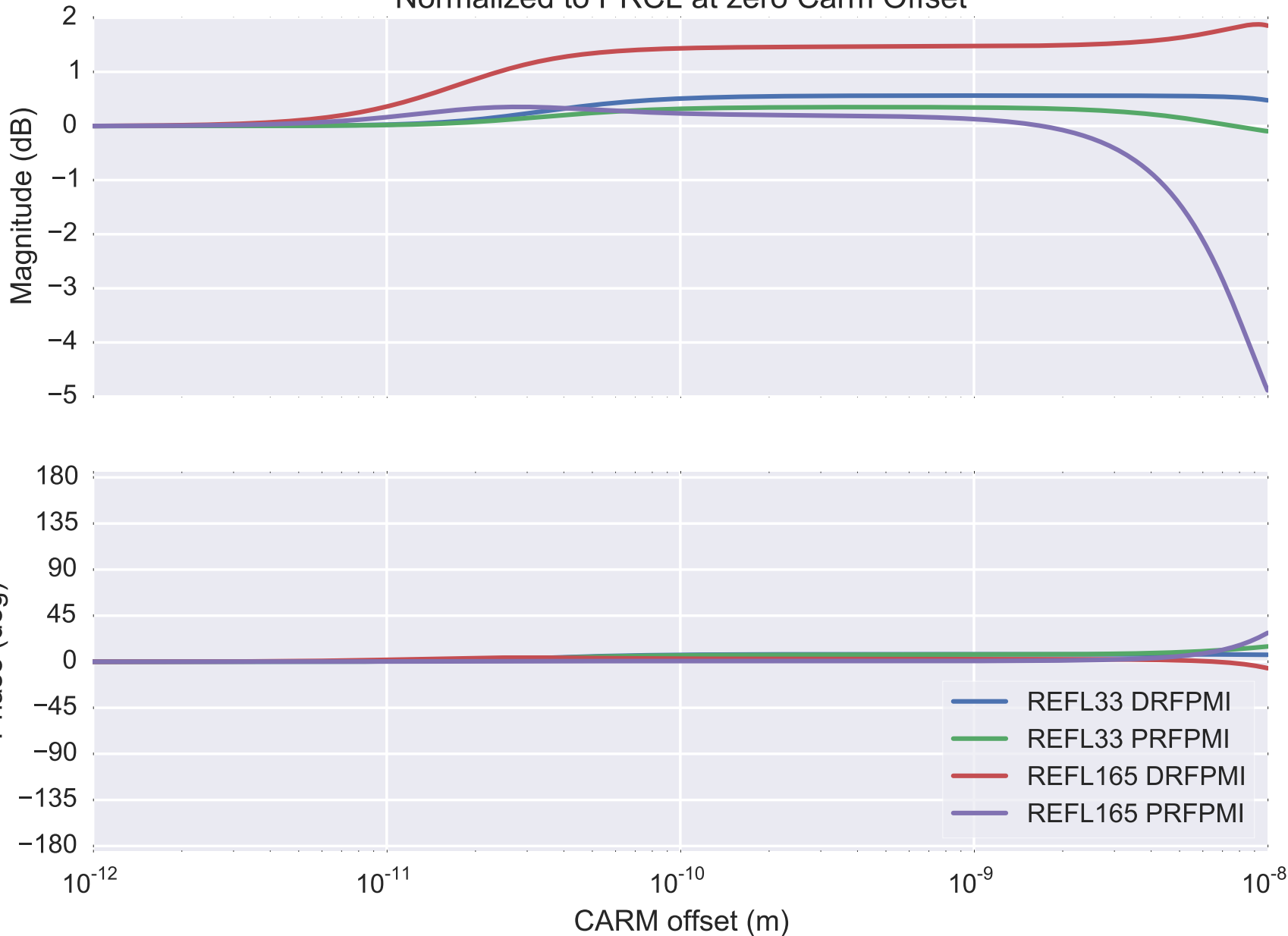
DC PRCL sensing in REFL 3F (Corrected SRC Length) Normalized to PRCL at zero Carm Offset
