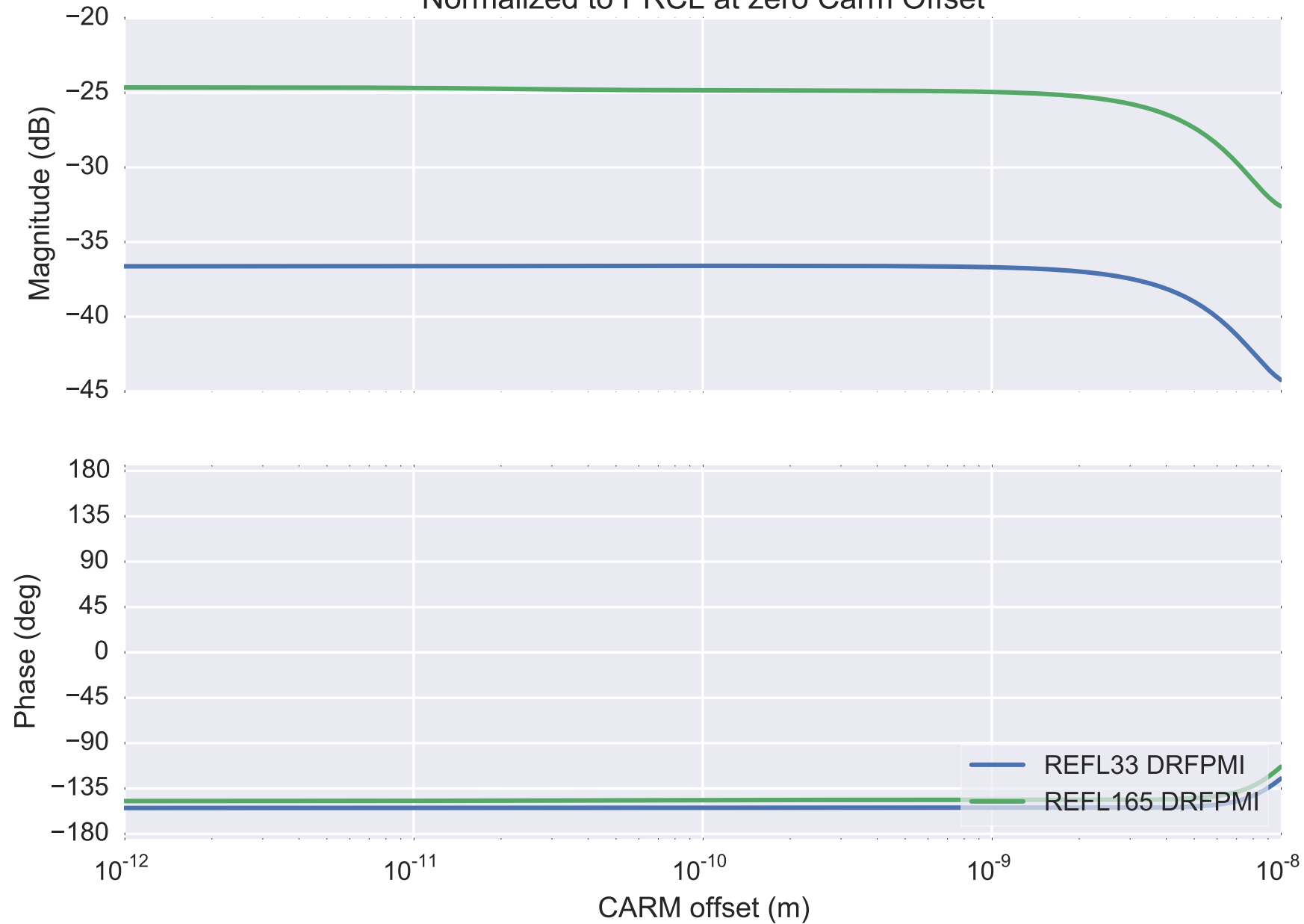
DC SRCL sensing in REFL 3F Normalized to PRCL at zero Carm Offset
