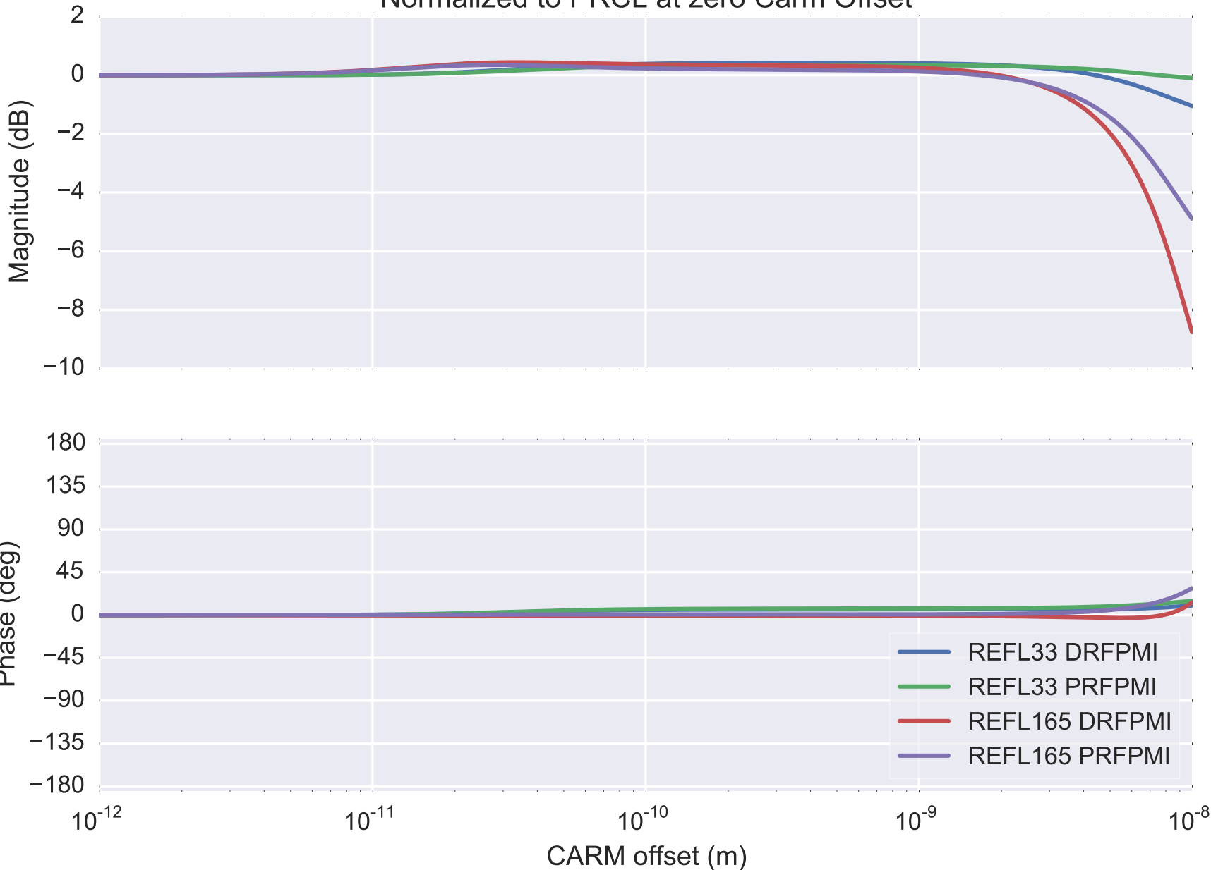
DC PRCL sensing in REFL 3F Normalized to PRCL at zero CARM Offset
