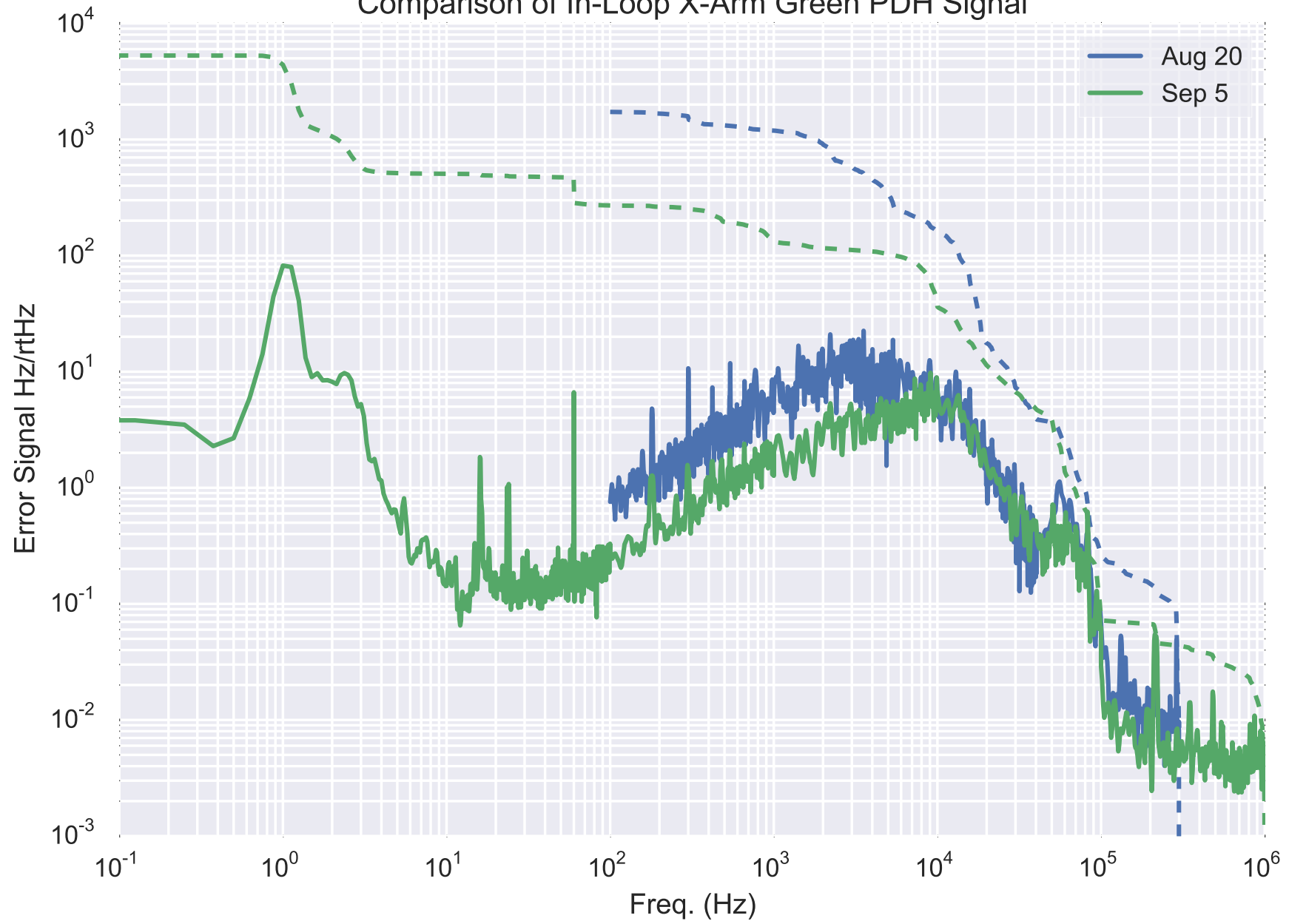
Comparison of In-Loop X-Arm Green PDH Signal
