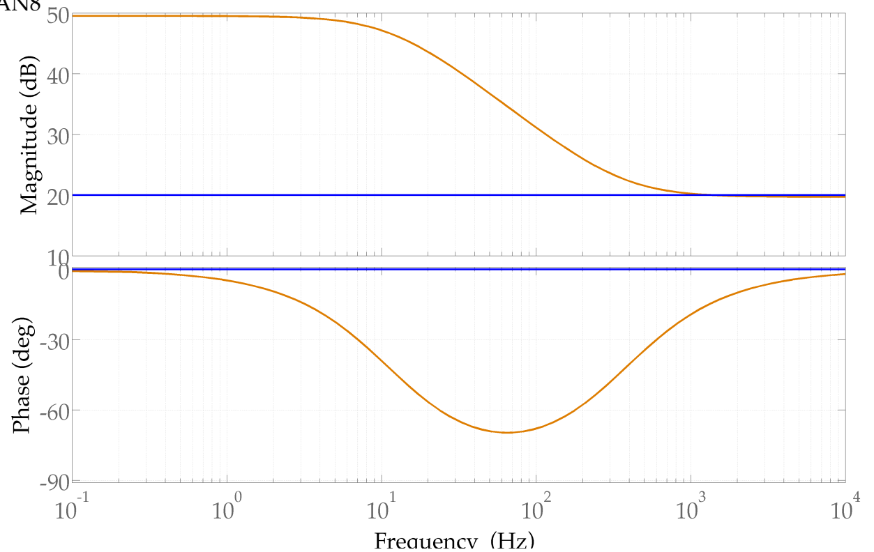
TF of boost Bode Diagram
