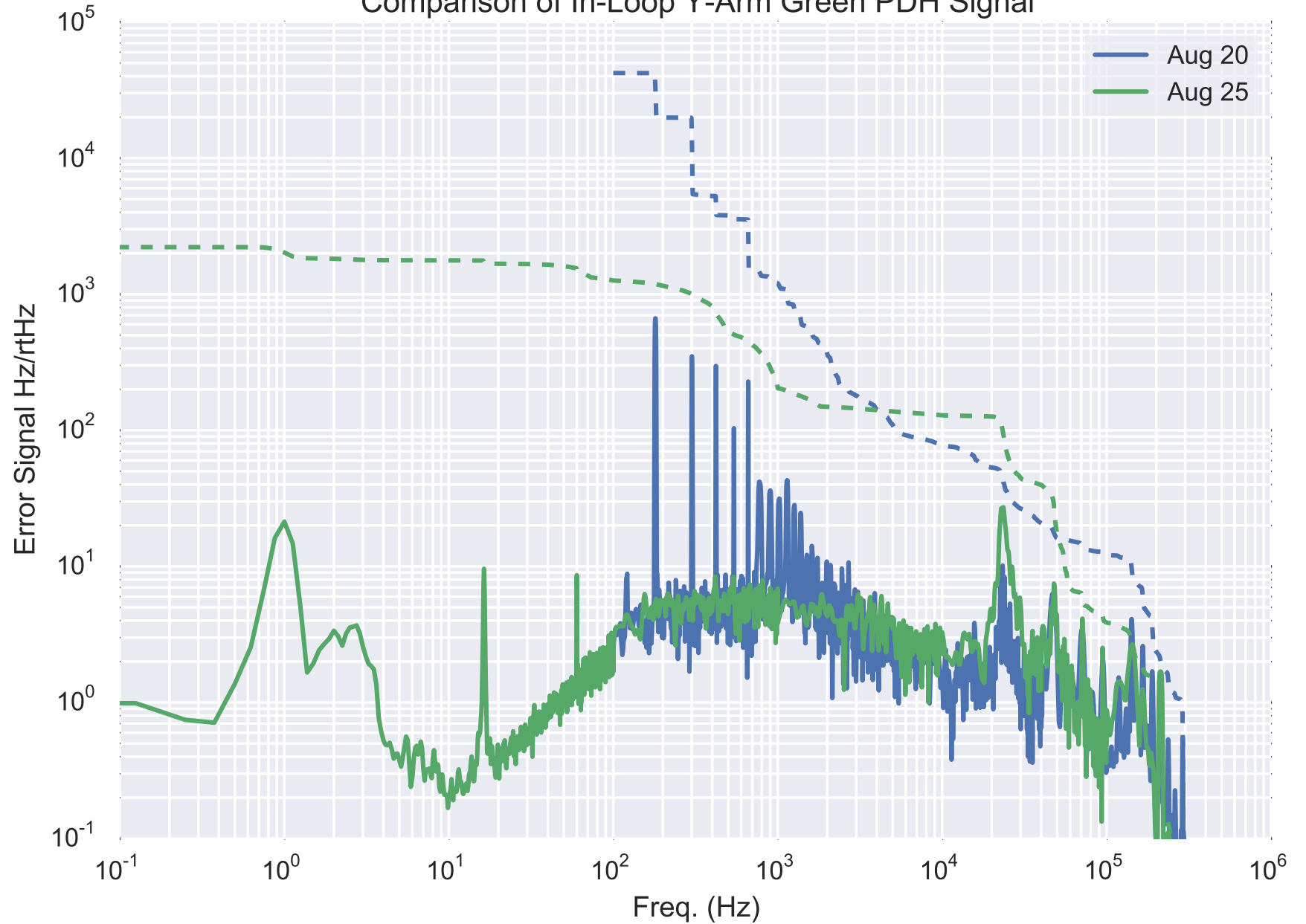
Comparison of In-Loop Y-Arm Green PDH Signal
