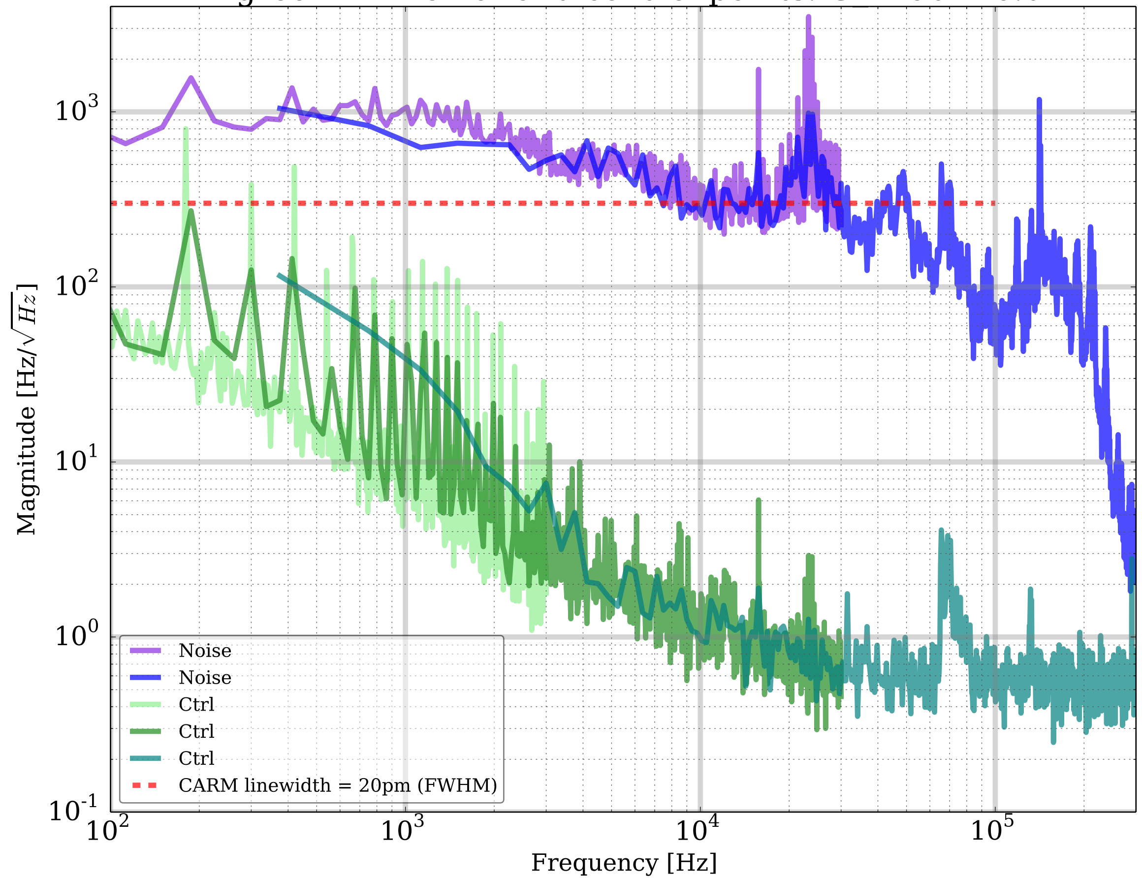
Y green PDH error and control points: G knob = 6.0
